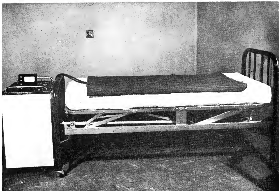
FIG. 1.—Photograph of the cooling apparatus. The refrigerating machine which cools the anti-freeze solution and pumps it through the blanket is shown at the left, and the large cooling blanket is spread out on the bed. The black box with the dial sitting on the refrigerating machine is the electrical thermometer.
